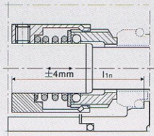
H76 单弹簧结构 d_1=14...100\text{mm} Dimensions, item no's and descriptions as for H7N, but with special single spring (item no. 1.5) for compensating large axial movements ( \pm 4\text{mm} )
