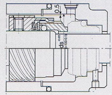
H7F 带螺纹泵 d_1 max. 100mm; Axial movement \pm 0.5\text{mm} . H75F d_1=28...200\text{mm} Axial movement 轴向窜动量 d_1 28...50=\pm 2\text{mm} d_1 58...100=\pm 3\text{mm} d_1 105...200=\pm 4\text{mm}
