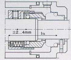
H75 多弹簧结构 d_1=28...200\text{mm} As H7N, but with multiple springs in sleeves (item no. 1.5) axial movements \pm 2 to 4 mm, dependent on diameter.
